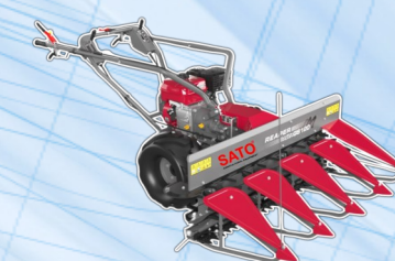
Rice Reaper GS-120 | 7.0HP
